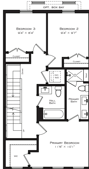
Alt Third Floor with 3 Bedrooms & Opt. Box Bay
